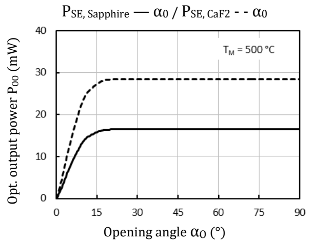
Optical output power ( P_{00} ) versus opening angle \alpha_0 (integral rotation of a cone) at 500^\circ\text{C } T_M
