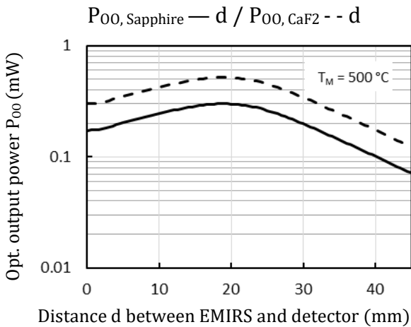
Optical output power ( P_{00} ) versus distance d of a 1 \text{ mm}^2 detection surface at 500^\circ\text{C } T_M
