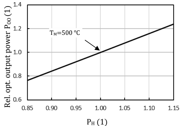
Relative change of optical output power ( P_{00} ) by changing heater power ( P_H )
