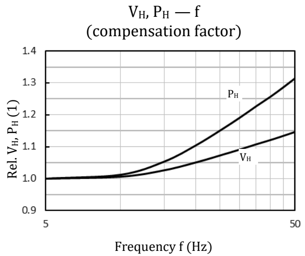
Relative (to RO) electrical drive values heater voltage V_H and power P_H versus frequency f for compensation
